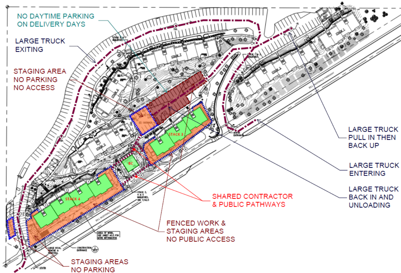
PW778A BW SIDING AND BRIDGES PHASE 1 - EXPECTATIONS AND IMPACTS CONSTRUCTION FENCING AND STAGING AREAS (APR 25 - JUN 10)
